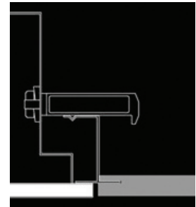
Concealed T Bar Ceiling Mounted in a concealed T bar ceiling, pushed up from below
